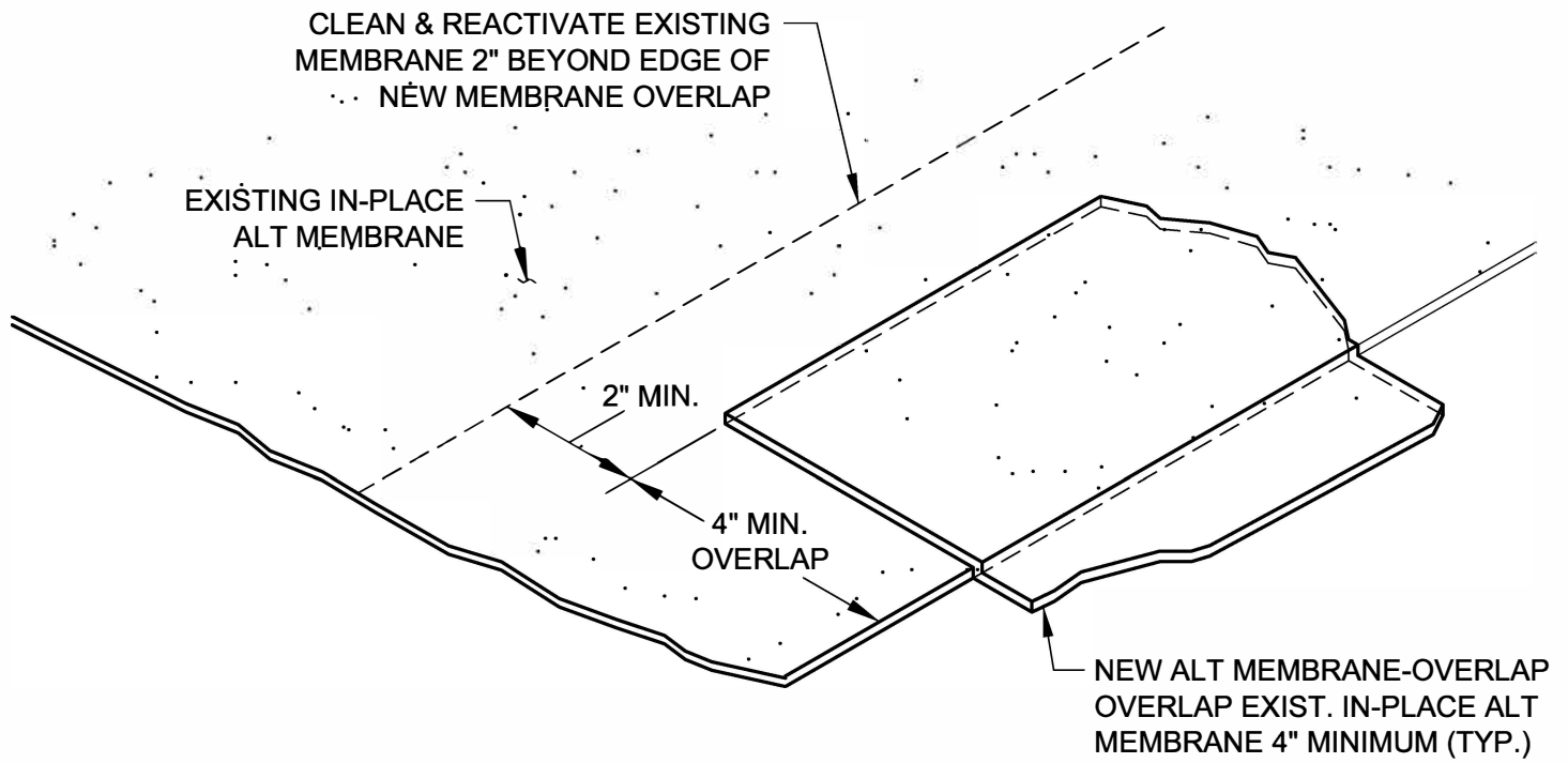
TIE-IN DETAIL SCALE: NTS
