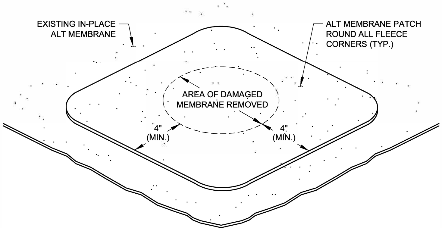
REPAIR DETAIL SCALE: NTS
